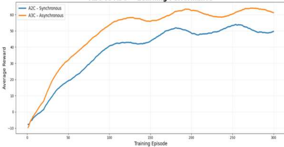
Fig 5: - A2c vs A3C Learning Performance
